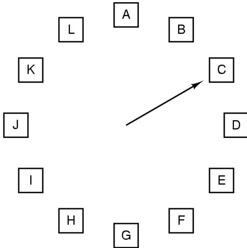
Figure 3-16. The clock page replacement algorithm.
